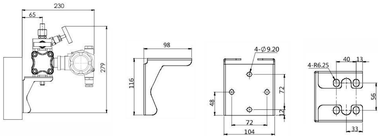
Installation dimensions of plate bending bracket
