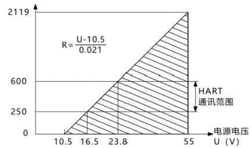
Figure 1. Power supply and load conditions
