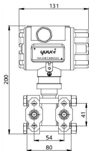
Overall size drawing with display function
